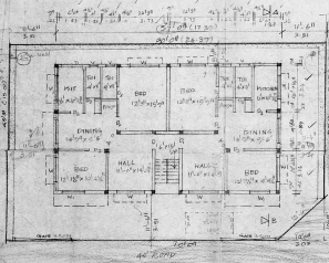
SITE GROUND FLOOR
