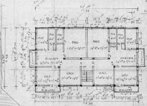
TYPICAL FLOOR FIRST AND SECOND
